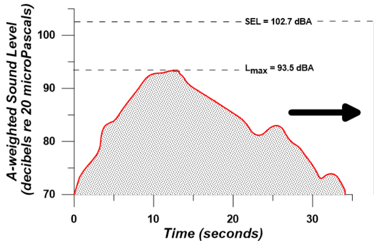
Figure D.2-4 Example Time History of Aircraft Noise Flyover
