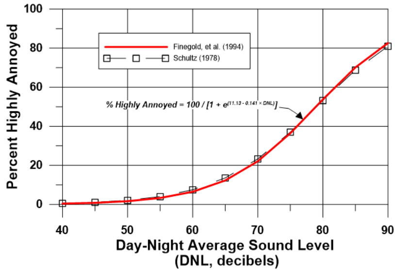
Figure D.2-8 Response of Communities to Noise; Comparison of Original Schultz (1978) with Finegold et al. (1994)
