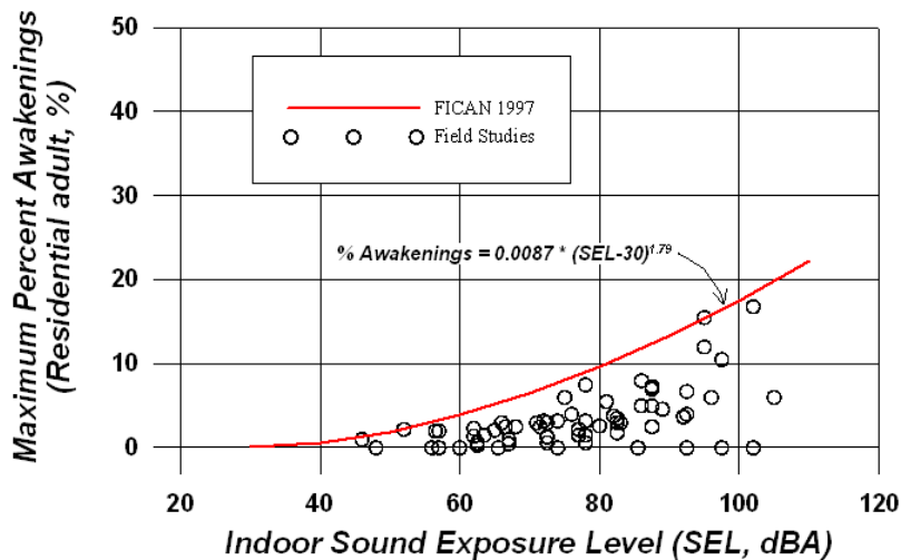
Figure D.2-11 Federal Interagency Committee on Aviation Noise 1997 Recommended Sleep Disturbance Dose-Response Relationship
