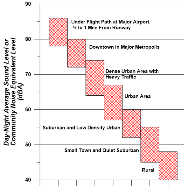
Figure D.2-6 Typical Day-Night Average Sound Level or Community Noise Equivalent Level Ranges in Various Types of Communities
